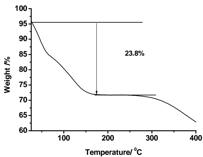
Figure S2. TGA of complex 1 .
