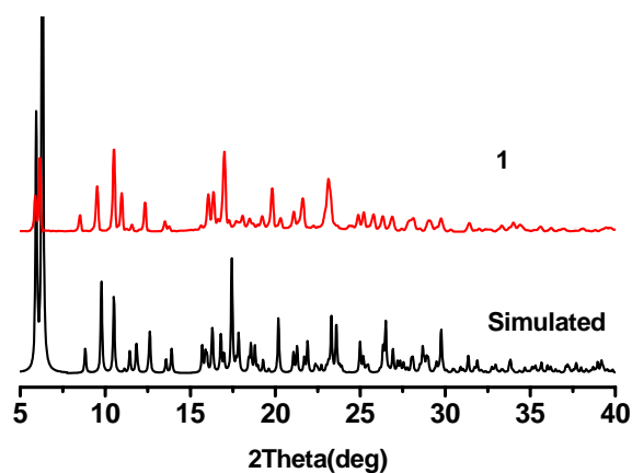
Figure S1. XRD pattern of 1 and the simulated pattern based on the single crystal 1 .
