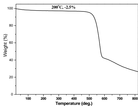
Fig. S1 TGA for complex 1 .
