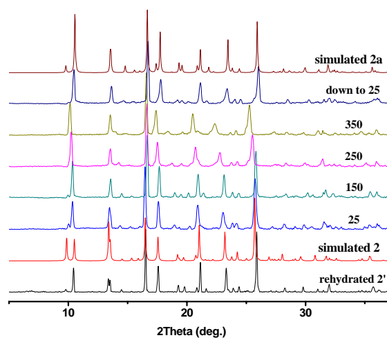
Fig. S5. Powder XRD patterns of the rehydrate 2' and 2 at different temperatures, and the simulated 2 and 2a based on the single crystal data.
