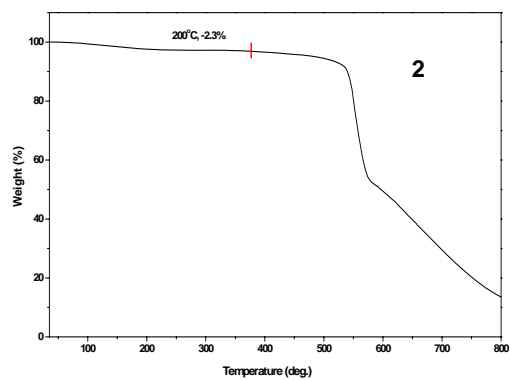
Fig. S3 TGA for complex 2 .
