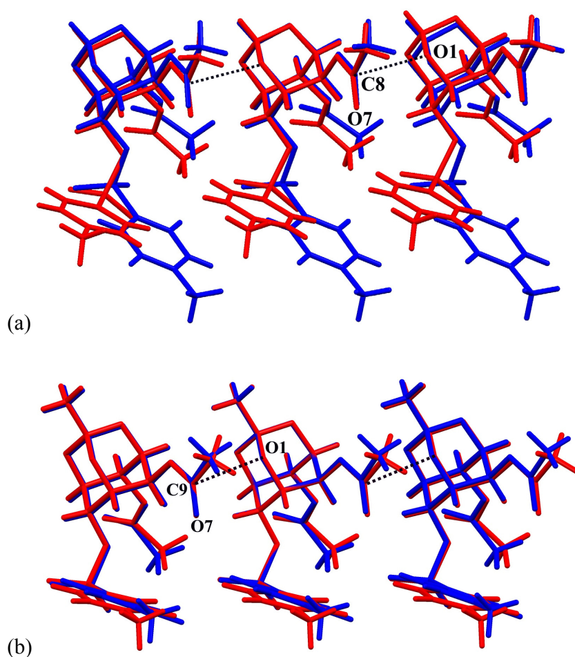
Figure S1: Molecular overlap figure of (a) dimorphs of 1 and (b) dimorphs of 2 [red: Form I; blue: Form II].
