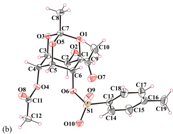
Figure S2: ORTEP of Form I crystals of (a) 1 and (b) 2 .
