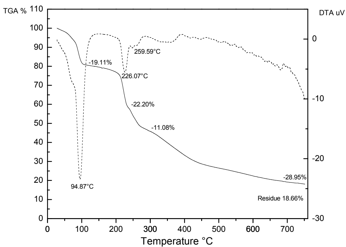
Figure S3. TGA and DTA curves for ZnB 2 Bipy·10H 2 O complex.
