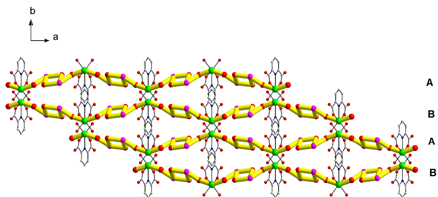
Figure S1 The packing structure of 8 with ABAB array along c axis. Color codes: green, Ce; purple, Ag; red, O; gray, C; blue, N; yellow lines, 1D CeAg 2 chains.
