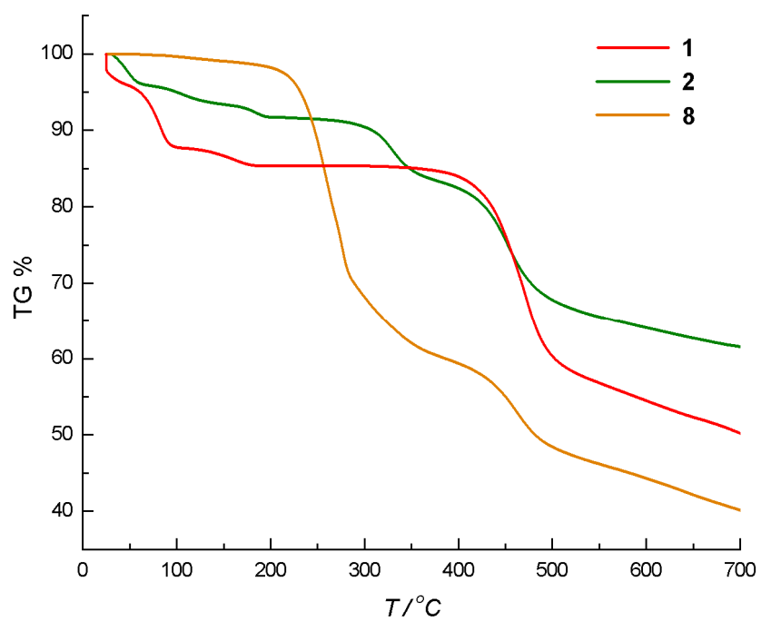
Figure S3 TGA diagrams for 1 , 2 and 8 .
