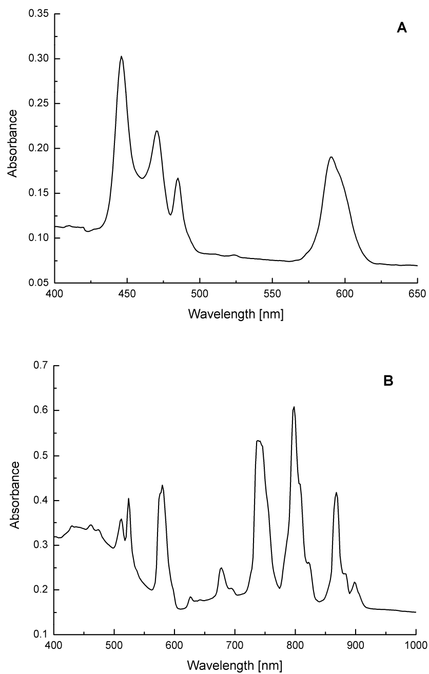
Figure S2 The UV/Vis absorption spectra of 1 (A) and 3 (B) in the solid state.
