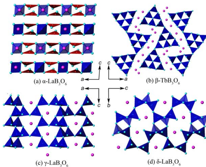
Figure S1. The structure of four polymorphs of LnB 3 O 6 .
