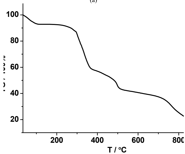
Fig. S1 TGA curves for 1 and 2.
