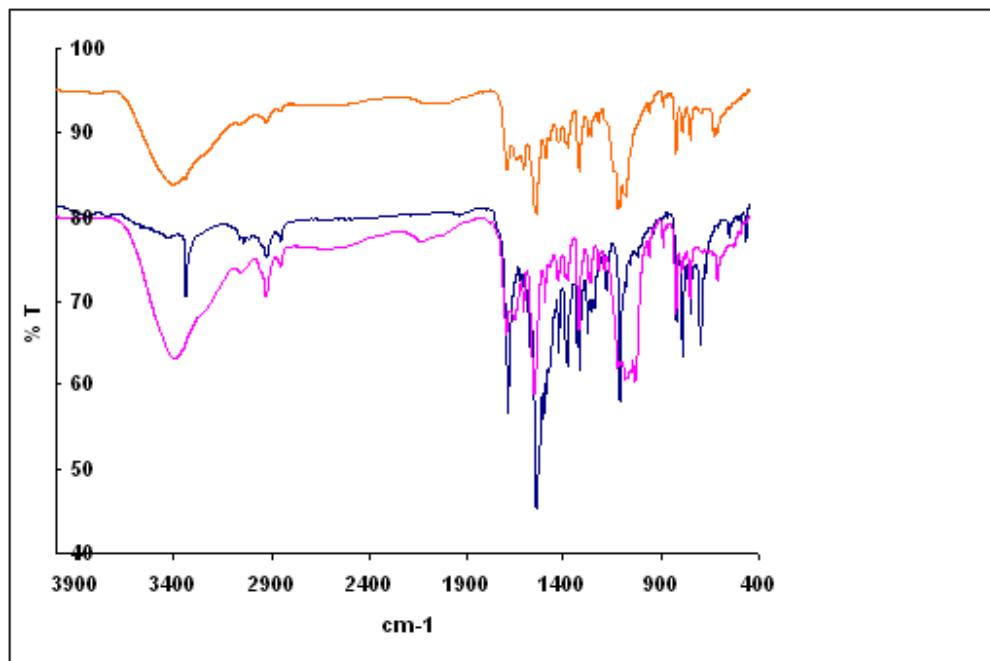
The IR (KBr, cm -1 ) of [N-(quinolin-8-yl)-2-(quinolin-8-yloxy)acetamide] (orange color) and its perchlorate salt IV (violet) and tetrafluoroborate salt V (Blue)
