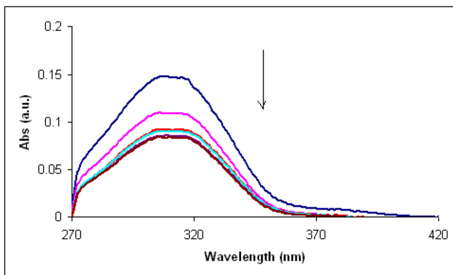
Decrease in absorbance in UV-spectra of a DMF solution of [N-(quinolin-8-yl)-2-(quinolin-8-yloxy)acetamide] on addition of solid sodium tetrafluoroborate
