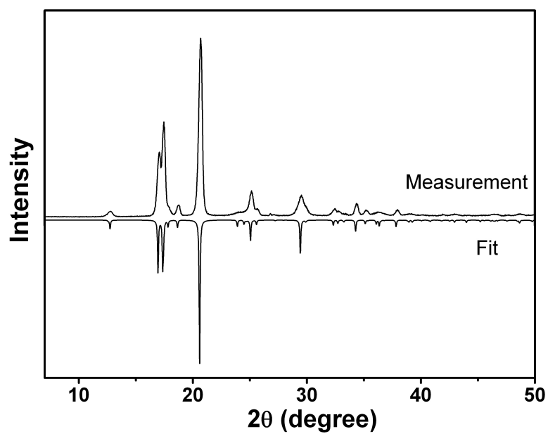
Fig. S1 The PXR diagram of compound I at room temperature.
