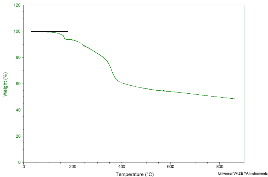
Figure S1. TGA curve for complex 2.
