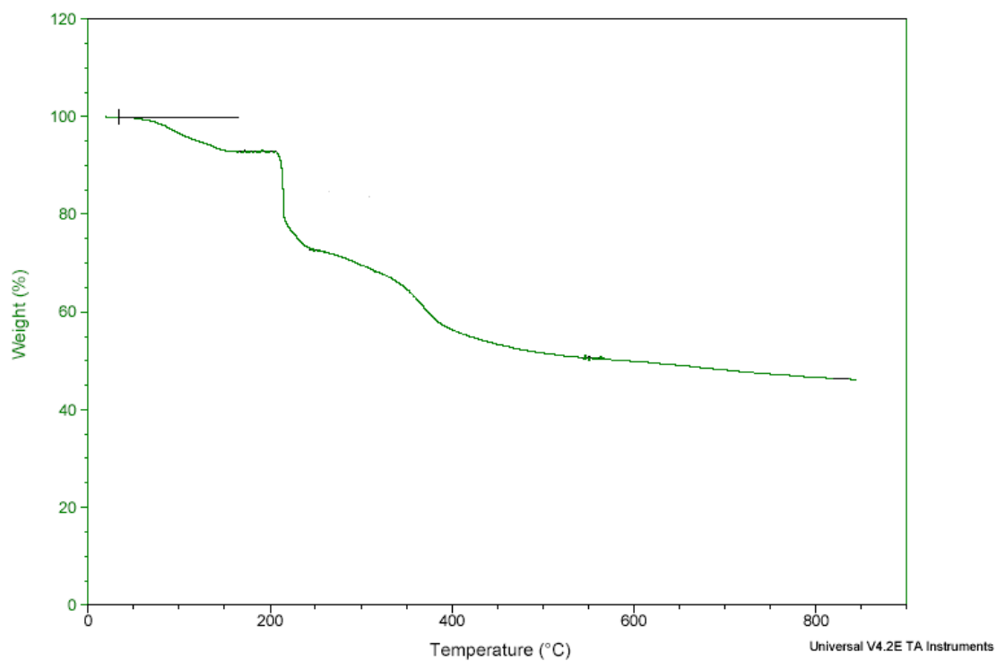
Figure S2. TGA curve of complex 3.
