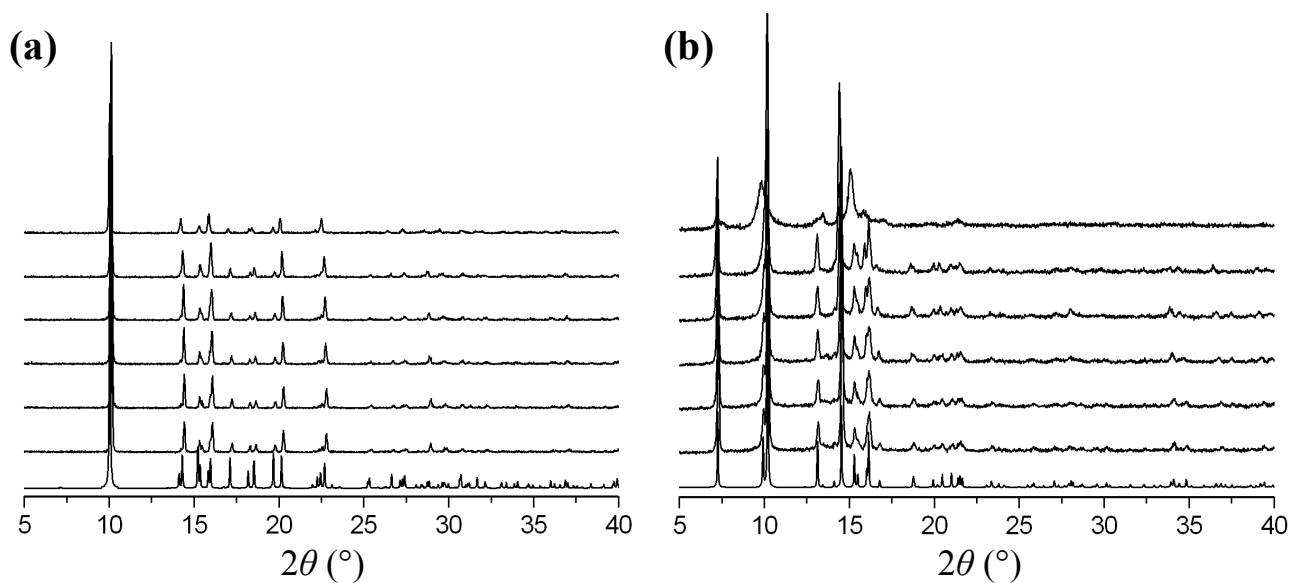
Fig. S2 Comparison plots of PXRD for (a) 1 and (b) 2 : (bottom to up) simulated and sample at room temperature, 50 °C, 100 °C, 150 °C, 200 °C, and 250 °C.
