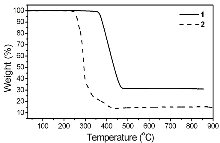
Fig. S1 Thermogravimetric (TG) traces of 1 and 2 .
