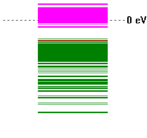
SI-Fig. 2. Calculated energy level of 2
