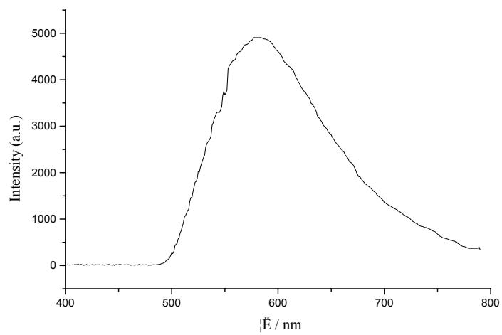
SI-Fig. 3. Emission spectra of the complex 6 (upon excitation at 330 nm) in dichloromethane solution at room temperature.
