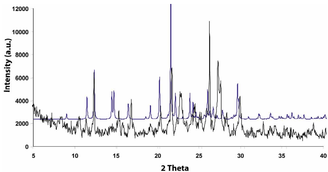
Fig : PXRD patterns of polymorph 1 (black = experimental, blue = simulated).
