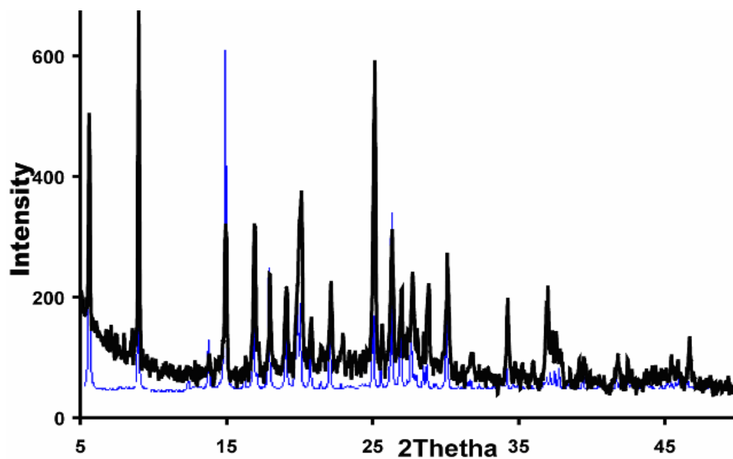
Fig. Powder diffraction pattern of polymorphs 4 (black = experimental; blue l = simulated)
