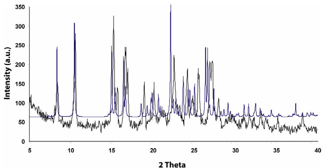
Fig : PXRD patterns of polymorph 2 (black = experimental, blue = simulated).
