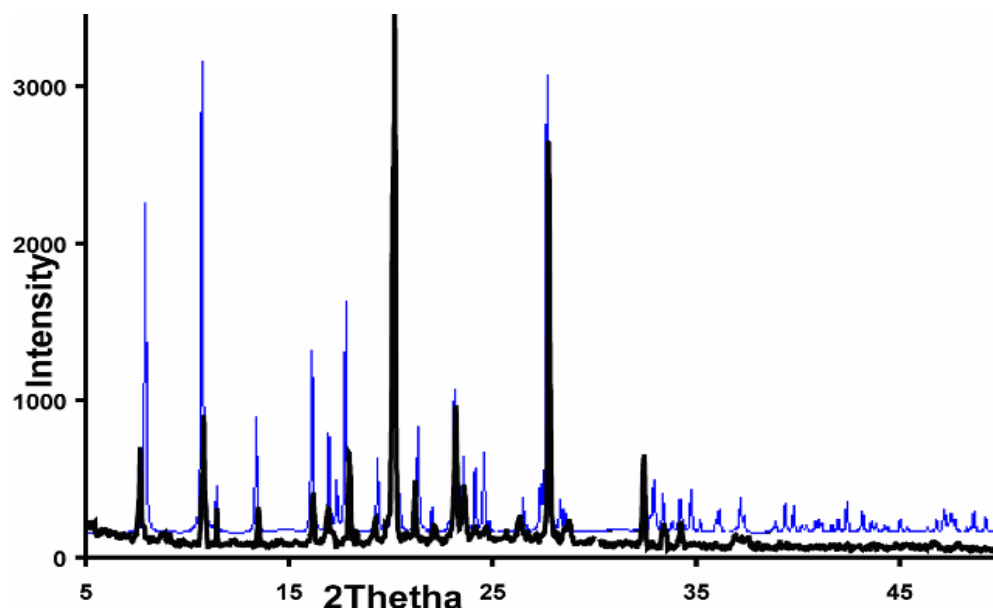
Fig : PXRD patterns of polymorph 2 (black = experimental, blue = simulated).
