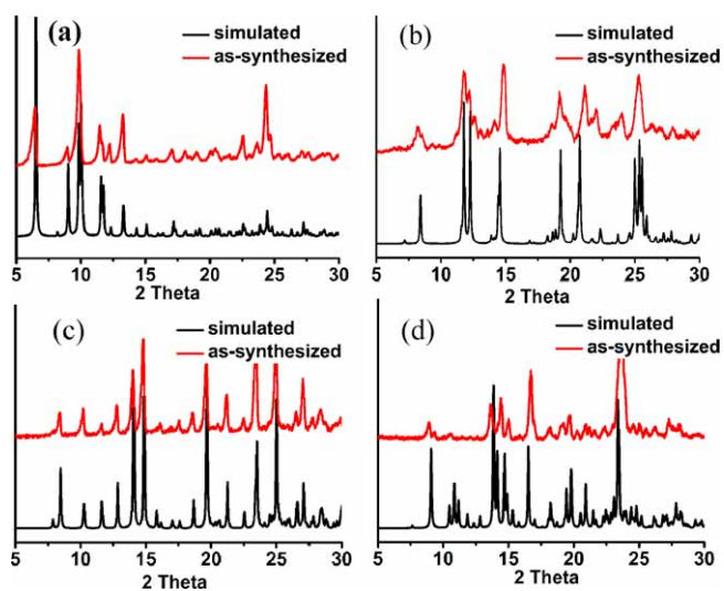
Fig. S1 Powder X-ray diffraction patterns of the compounds: as-synthesized (red) and simulated from the single-crystal diffraction data (black): (a) 1 ; (b) 2 ; (c) 3 ; (d) 4 .
