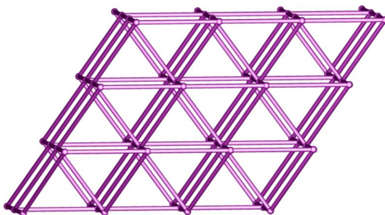
Fig. S3. Schematic view of the net topology of 1 If the dimeric [\text{Cu}(\text{COO})_2] units can be considered as the nodes.
