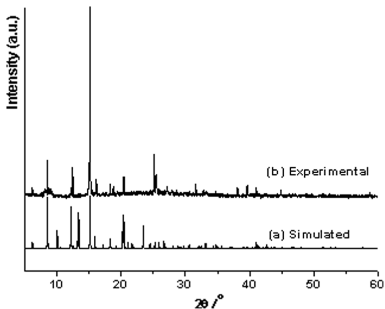
Fig. S2 The experimental and simulated PXRD patterns for complex 2.
