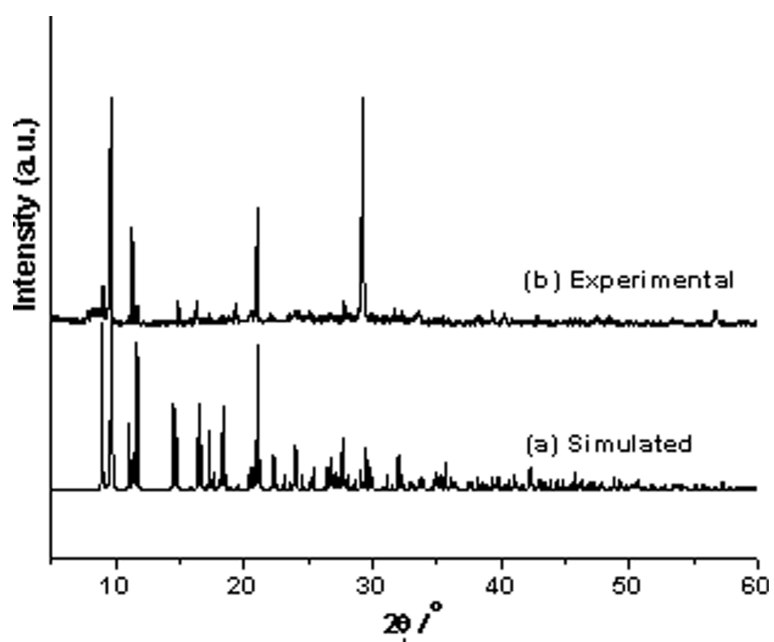
Fig. S4 The experimental and simulated PXR D patterns for complex 4.
