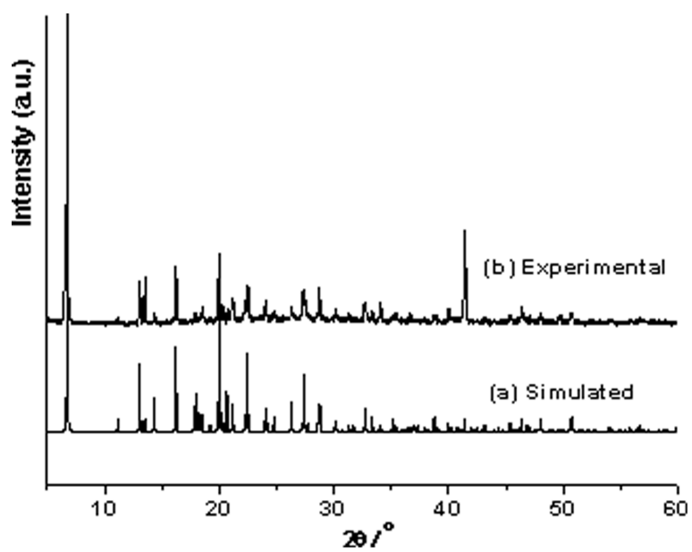
Fig. S3 The experimental and simulated PXR D patterns for complex 3.
