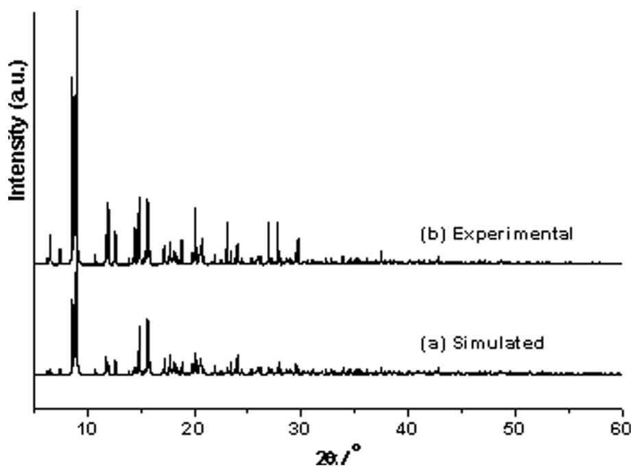
Fig. S5 The experimental and simulated PXR D patterns for complex 5.
