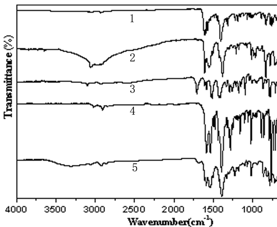
Fig. S6 IR spectra of complexes 1-5.
