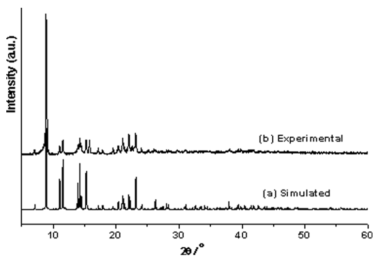
Fig. S1 The experimental and simulated PXRD patterns for complex 1.
