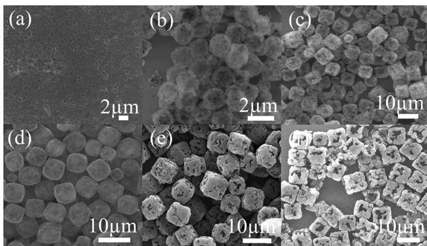
Figure S2 SEM images of morphology evolution of TBPe microcube at different time: a) 1min, b) 20min, c) 40min, d) 4h, e) 8h, f) 20h
