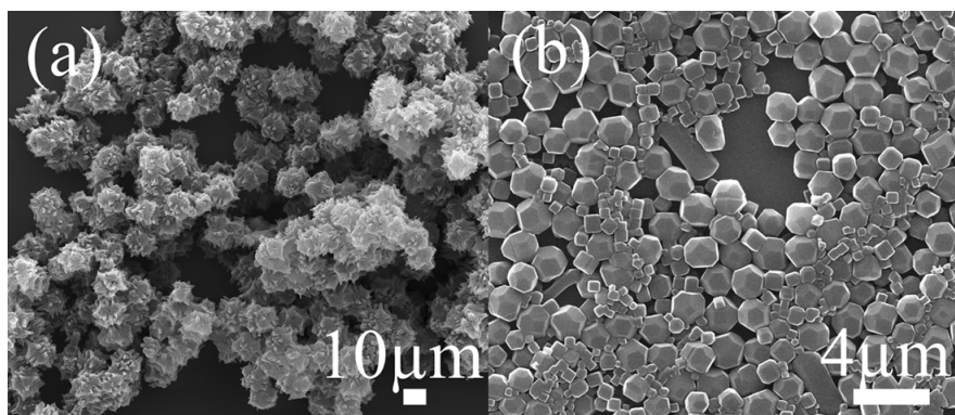
Figure S1 SEM images of products that both nucleation and growth temperature are kept at (a) 6°C (b) 25°C
