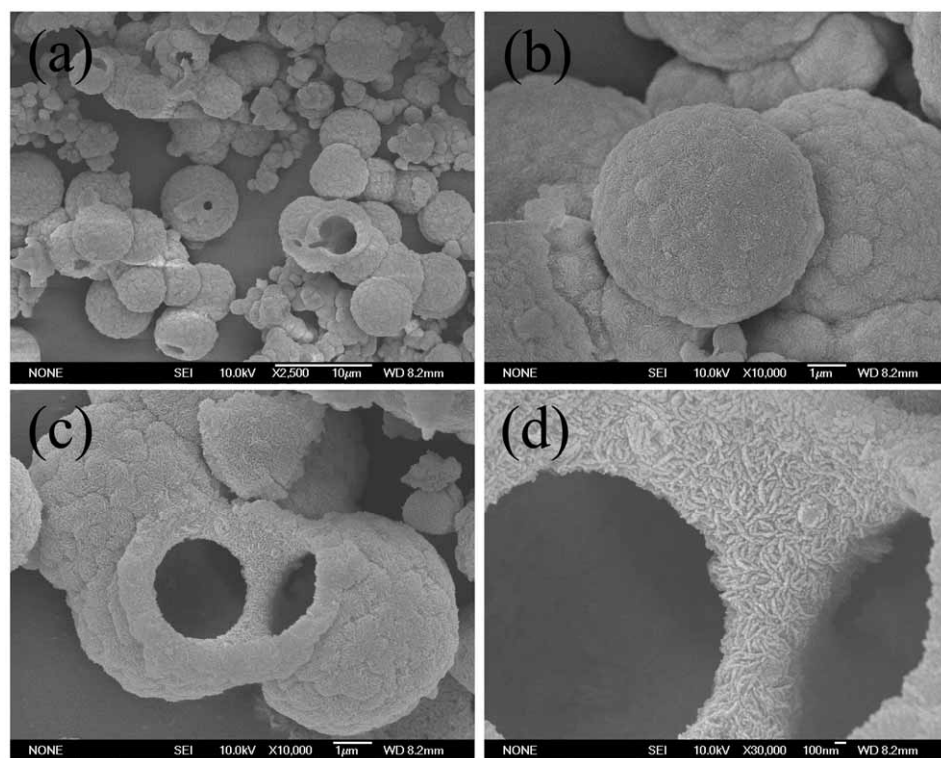
Figure S1. Low- and high- magnification SEM images of hollow microspheres prepared under pH=3.
