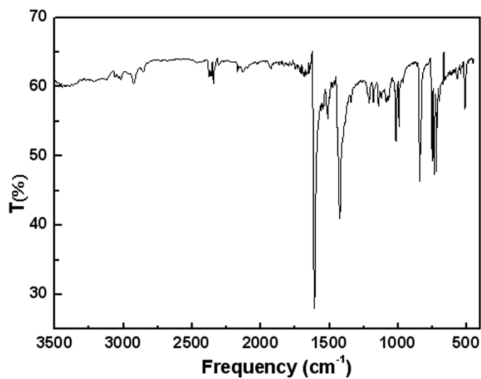
Figure S2. FT-IR spectroscopic characterization for complex 2.
