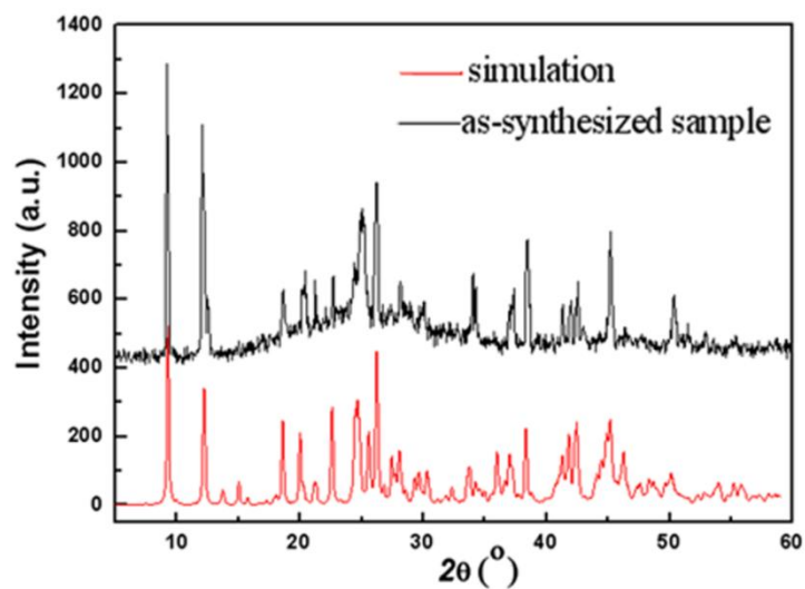
Figure S3. XRPD patterns of simulated from a single crystal of complex 1 (red), and as-synthesized sample of complex 1 (dark).
