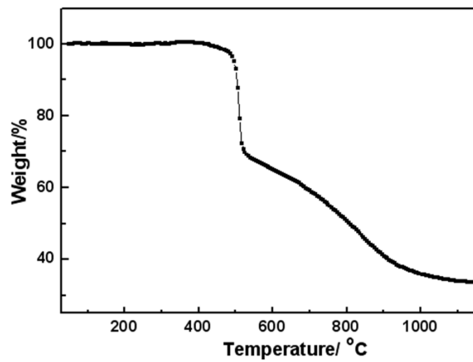
Figure S6. TGA profile for complex 2.
