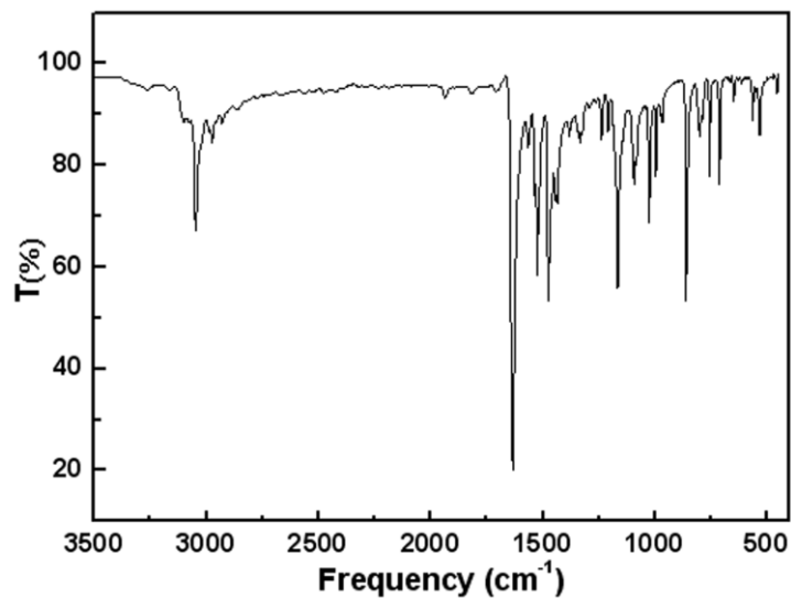
Figure S1. FT-IR spectroscopic characterization for complex 1.
