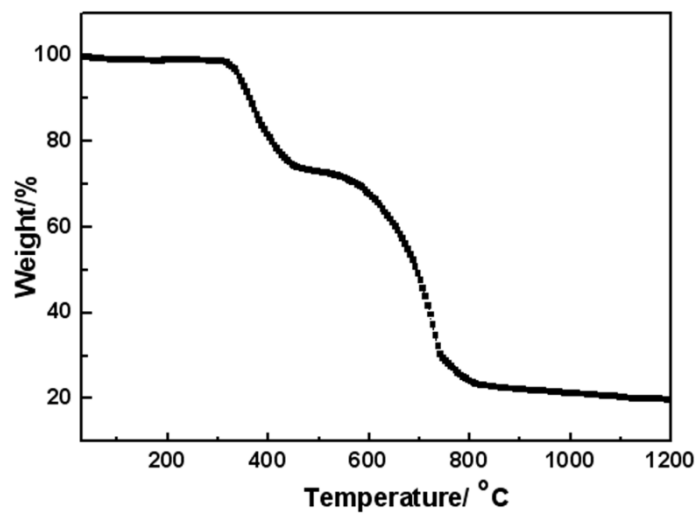
Figure S5. TGA profile for complex 1.
