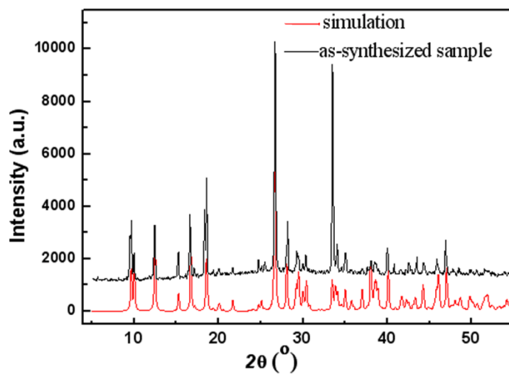
Figure S4. XRPD patterns of simulated from a single crystal of complex 2 (red), and as-synthesized sample of complex 2 (dark).
