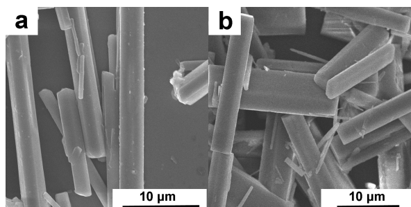
Fig. S2. SEM image of TbDBM-MW (a) and SmDBM-MW (b) synthesized by 0.5 mL water.
