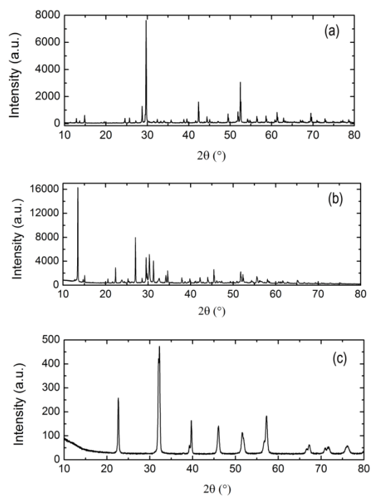
Fig. S1 XRD patterns of as-obtained K_xBi_{1-x}FeO_{3-y} nanowires (a), microrods (b) and BiFeO_3 nanoparticles (c).
