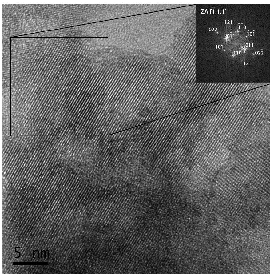
Fig. SI - HR-TEM image and FFT patterns of FeWO 4 nanocrystals obtained at 170°C for 45 min with PEG-200 non-ionic surfactant.
