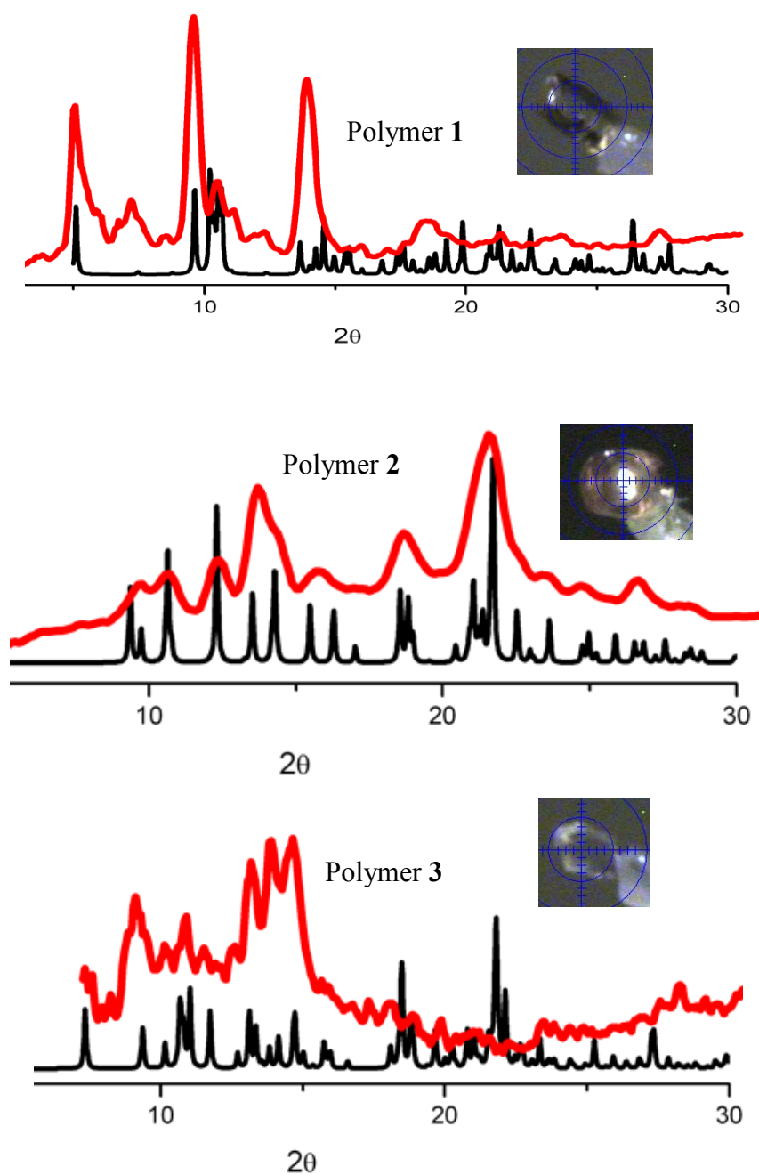
Figure S1. The experimental XRD patterns/red and the simulated XRD patterns/black from the single crystal data of 1-3. The inset is the shape of the single crystal of 1-3.
