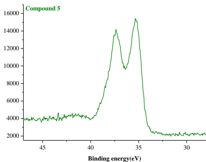
Fig. S5 The XPS spectra for compound 1-6.
