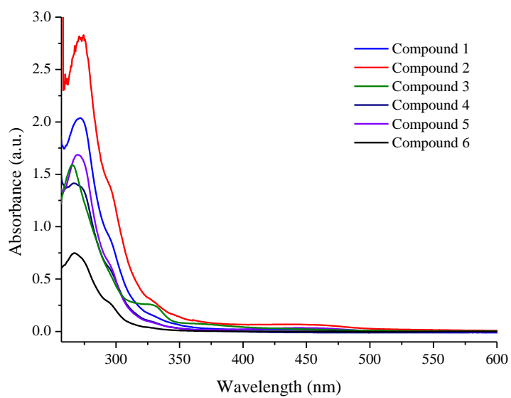
Fig. S1 The UV-Vis spectra for compound 1-6.
