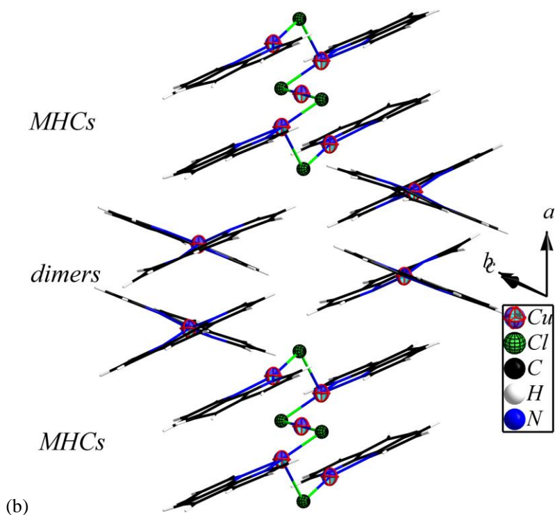
Fig. S2 (a) The upper view of the representation of the supramolecular infinite straight column structure along a axis constructed from metal halide clusters and supramolecular dimers. (b) The side view of the supramolecular column.
