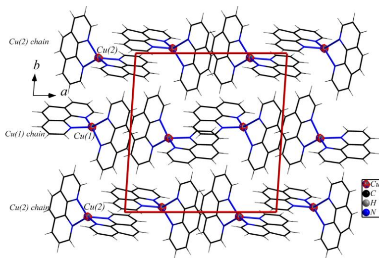
Fig. S3 The arrangement of the supramolecular chains based on Cu(1) and Cu(2) TMCs in compound 5.
