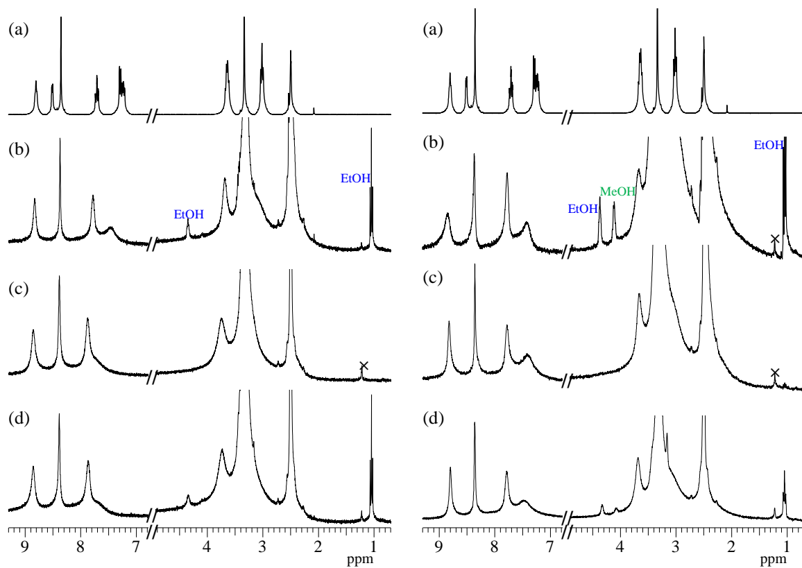
Fig. S2. ^1\text{H} NMR spectra ( \text{DMSO-}d_6 ) during the evacuation of re-absorption of the solvated molecules into [\text{Cu}_3\text{X}_6\text{L}_2] . Left: L (a), 6\text{EtOH}@[\text{Cu}_3\text{Cl}_6\text{L}_2] (b), evacuated sample at 80\text{ }^\circ\text{C} overnight (c), and re-absorbed sample (d); right: L (a), 3\text{MeOH}\cdot 3\text{EtOH}@[\text{Cu}_3\text{Br}_6\text{L}_2] (b), evacuated sample at 80\text{ }^\circ\text{C} overnight (c), and re-absorbed sample (d).
