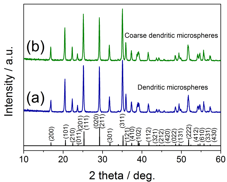
Fig. S1 XRD patterns of the dendritic microspheres and the coarse dendritic microspheres.
