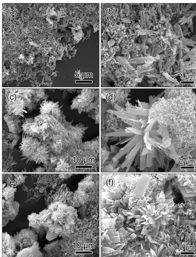
Fig. S2 SEM images of the LiMnPO 4 /C composites with different morphologies obtained after the ball milling and the calcination: the dispersed wedges (a and b); the dendritic microspheres (c and d); the coarse dendritic microspheres (e and f).
