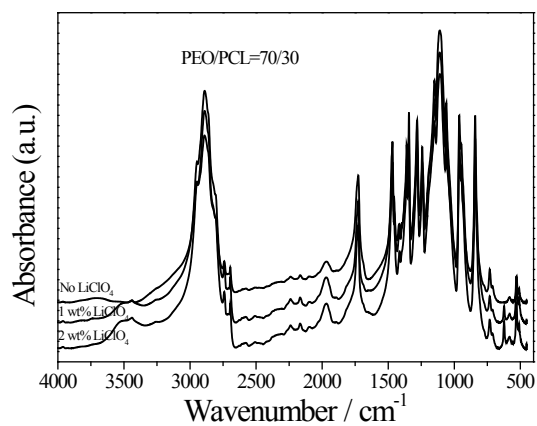
Fig S2. Infrared spectra for PEO/PCL/LiClO 4 ternary blend with PEO/PCL=70/30, the concentration of LiClO 4 changes from 0 to 2 wt%.
