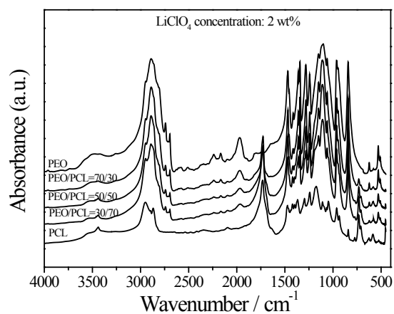
Fig S1. Infrared spectra for PEO/PCL/LiClO 4 ternary blend with different PEO/PCL ratios, the concentration of LiClO 4 is fixed at 2 wt%.
