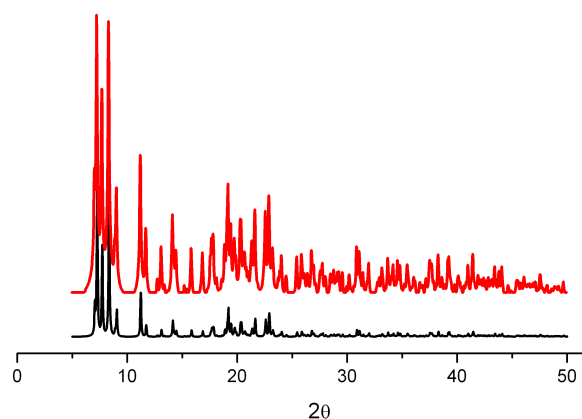
Figure S1. For 2 , the plots of PXRD patterns for the data simulated from the single crystal data (black) and the experimental data (red).
