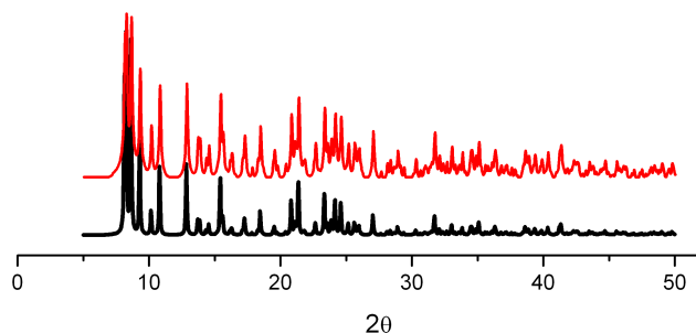
Figure S1. For 1 , the plots of PXRD patterns for the data simulated from the single crystal data (black) and the experimental data (red).
