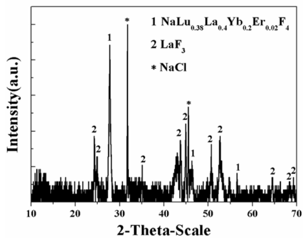
Fig. S1 The XRD patterns of \text{NaLu}_{0.38}\text{La}_{0.4}\text{Yb}_{0.2}\text{Er}_{0.02}\text{F}_4 NCs.
