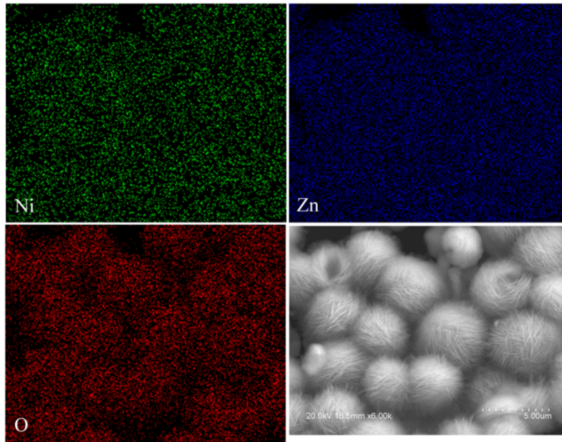
Fig. S2 EDS spectra measurements of P2.
