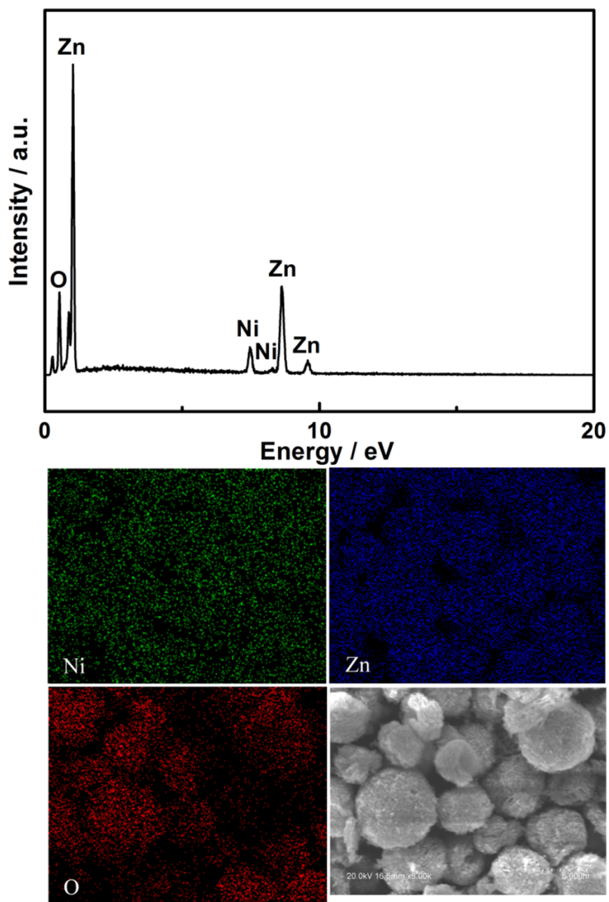
Fig. S3 EDS spectra measurements of P3.
