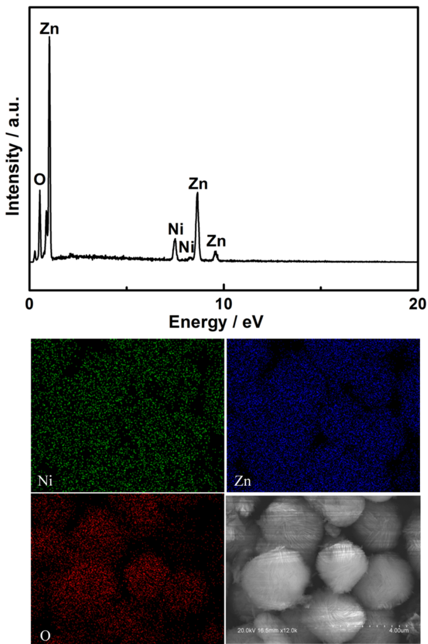
Fig. S1 EDS spectra measurements of P1.
