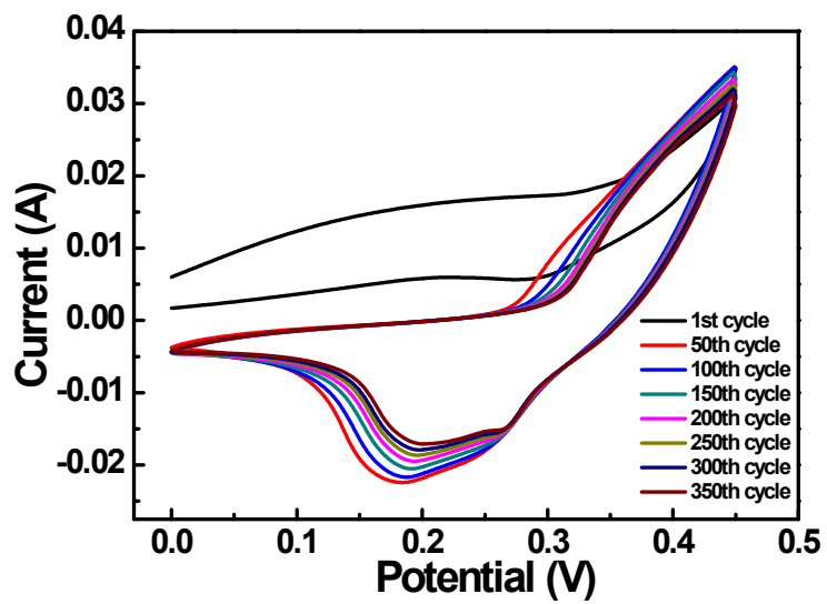
Fig. S2 Cycling stability of FeCl 3 pseudocapacitor at the scan rate of 10 mV/s.
