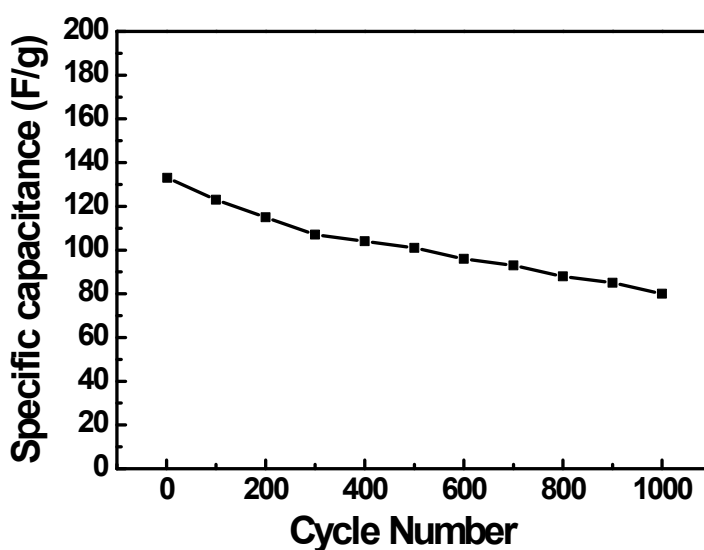
Fig. S1 Cycling stability of FeCl 3 pseudocapacitor at the current density of 30A/g.
