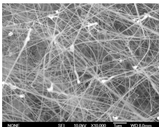
Fig. S2 The SEM image of SiC nanowires on Si substrate by using \text{Ni}(\text{NO}_3)_2 (0.04M) as catalyst
