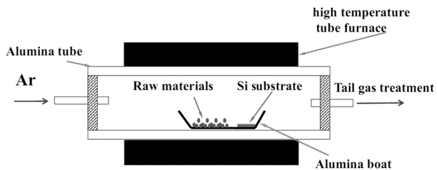
Fig. S1 The schematic diagram of the reactor system
