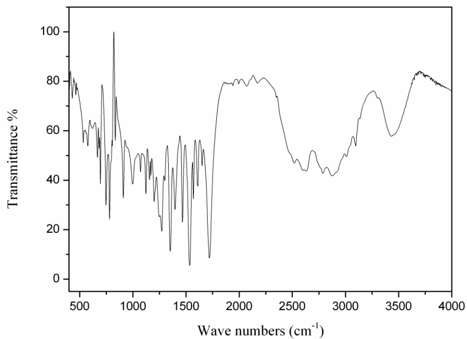
The IR curve of 5
