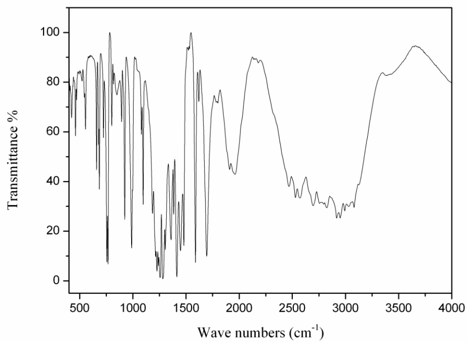
The IR curve of 8
