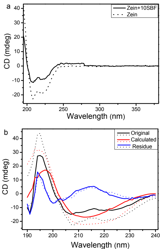
Figure S1. (a) CD spectra of 1mg/mL zein solution before (dot line) and after (solid line) interacted with 10 SBF and (b) their simulation results with JWS program.
