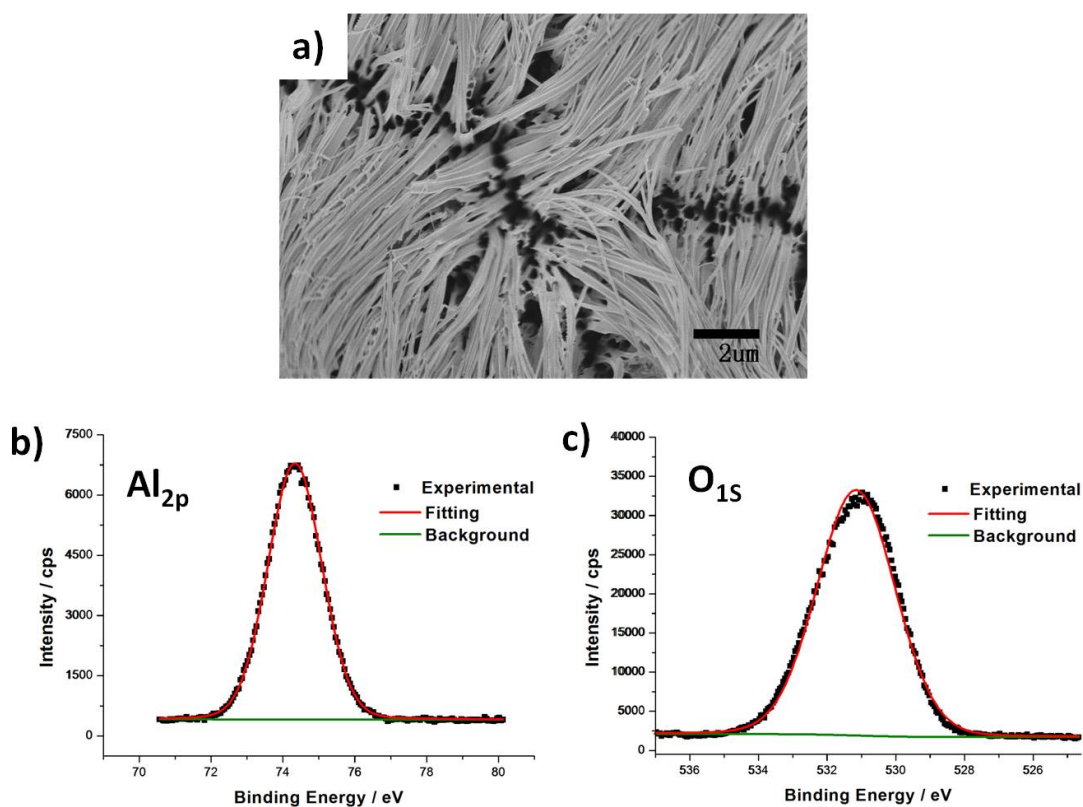
Figure S1: a) high magnified SEM image of the as-prepared alumina nanowires. b) and c) X-ray photoelectron Spectroscopy of the as-prepared alumina nanowires, and the characteristic peaks of Al 2p and O 1s were clearly observed.
