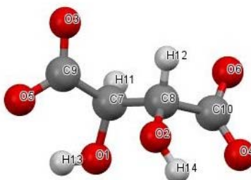
Fig. S1. Tartrate molecule structure and atom names.
