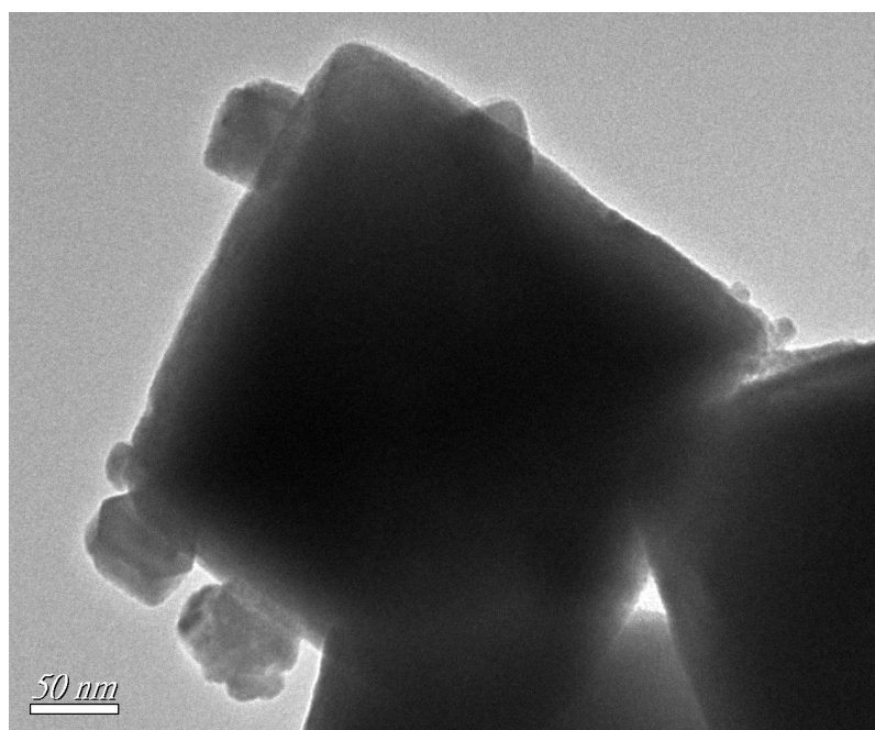
Figure 2 TEM image of \text{Ag/Bi}_{3.84}\text{W}_{0.16}\text{O}_{6.24} nanooctahedrons after 3 photocatalytic cycles
