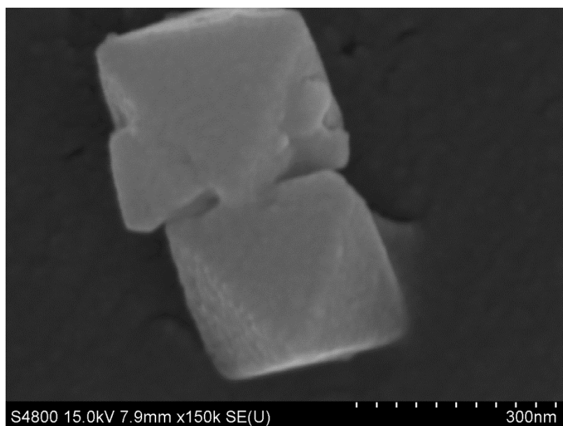
Figure 1 SEM image of \text{Ag/Bi}_{3.84}\text{W}_{0.16}\text{O}_{6.24} nanooctahedrons after 3 photocatalytic cycles
