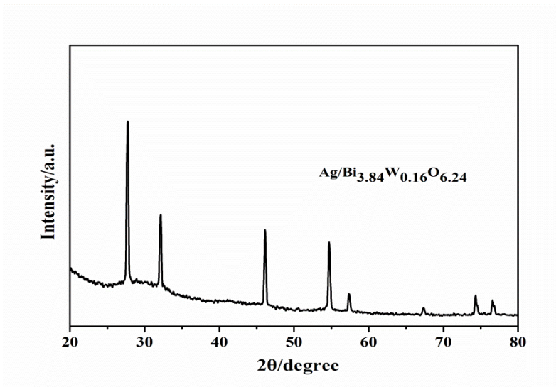
Figure 3 XRD pattern of Ag/Bi 3.84 W 0.16 O 6.24 nanooctahedrons after 3 photocatalytic cycles
