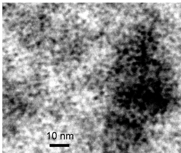
Fig. S1 TEM image of diop modified Pt nanoclusters.
