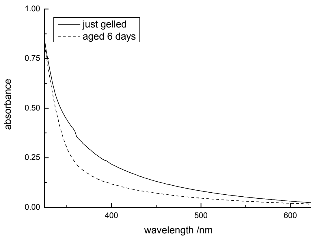
Supplementary figure S1. Absorption spectrum for Eu POM in a sol-gel derived matrix with aging time.
