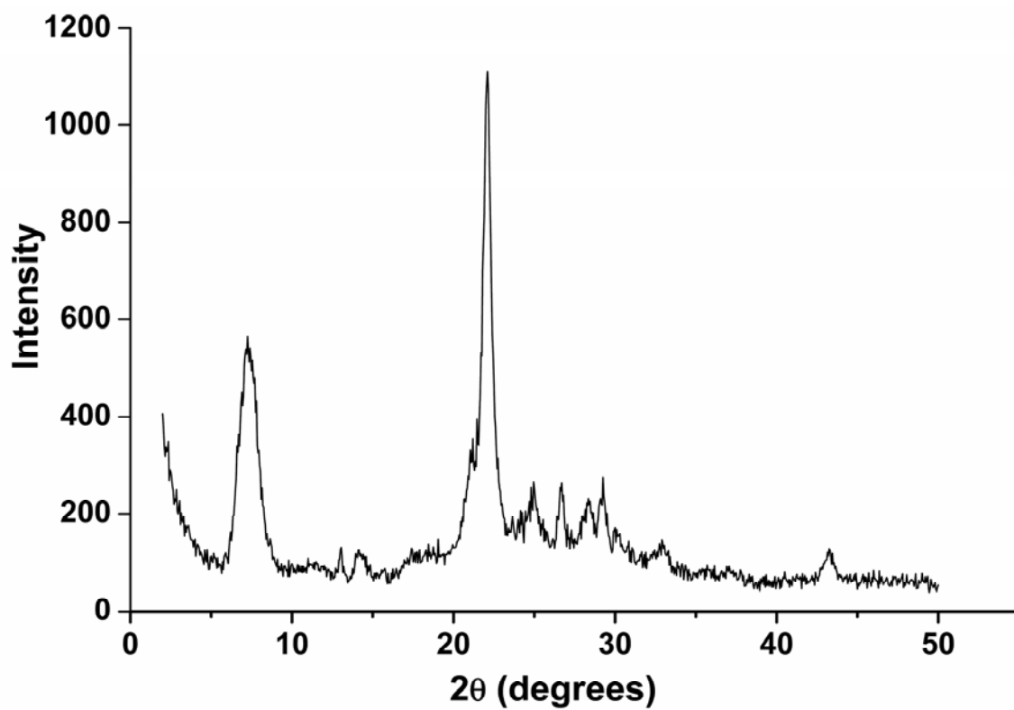
Fig.: XRD pattern of zeolite NH 4 BEA.
