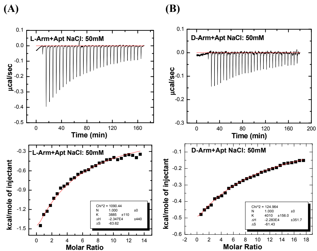
Figure S3. The ITC profiles at 10mM phosphate buffer, 50mM NaCl, pH 6.5, 20°C (A) L-Arm (B) D-Arm
