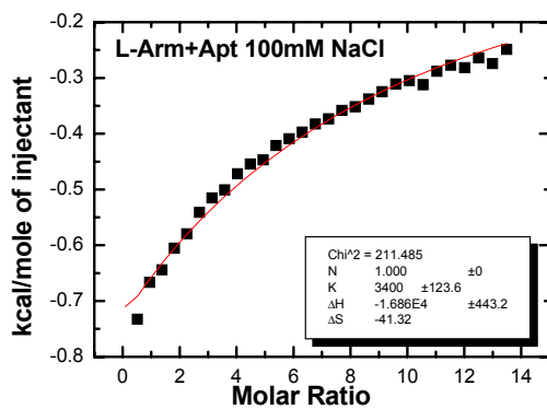
Figure S4. The ITC profiles at 10mM phosphate buffer, 100mM NaCl, pH 6.5, 20°C (A) L-Arm (B) D-Arm
