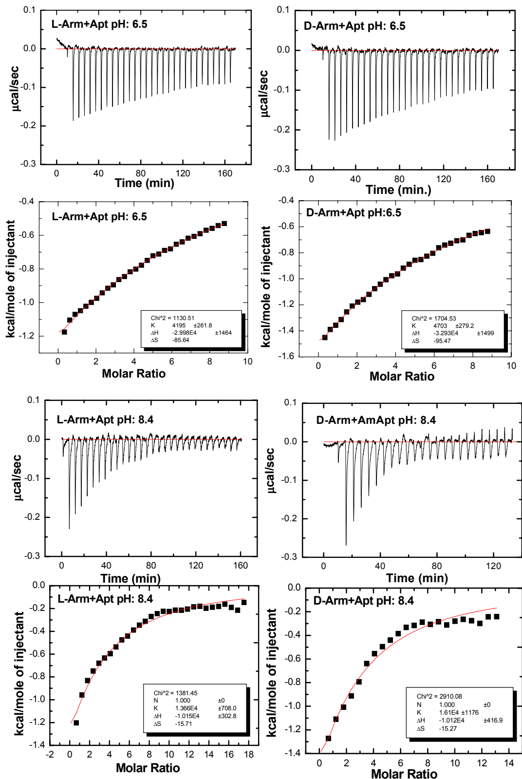
Figure S4. The ITC profiles at 10mM phosphate buffer, 100mM NaCl, pH 6.5 & 8.4 , 20°C (A) L-Arm (B) D-Arm
