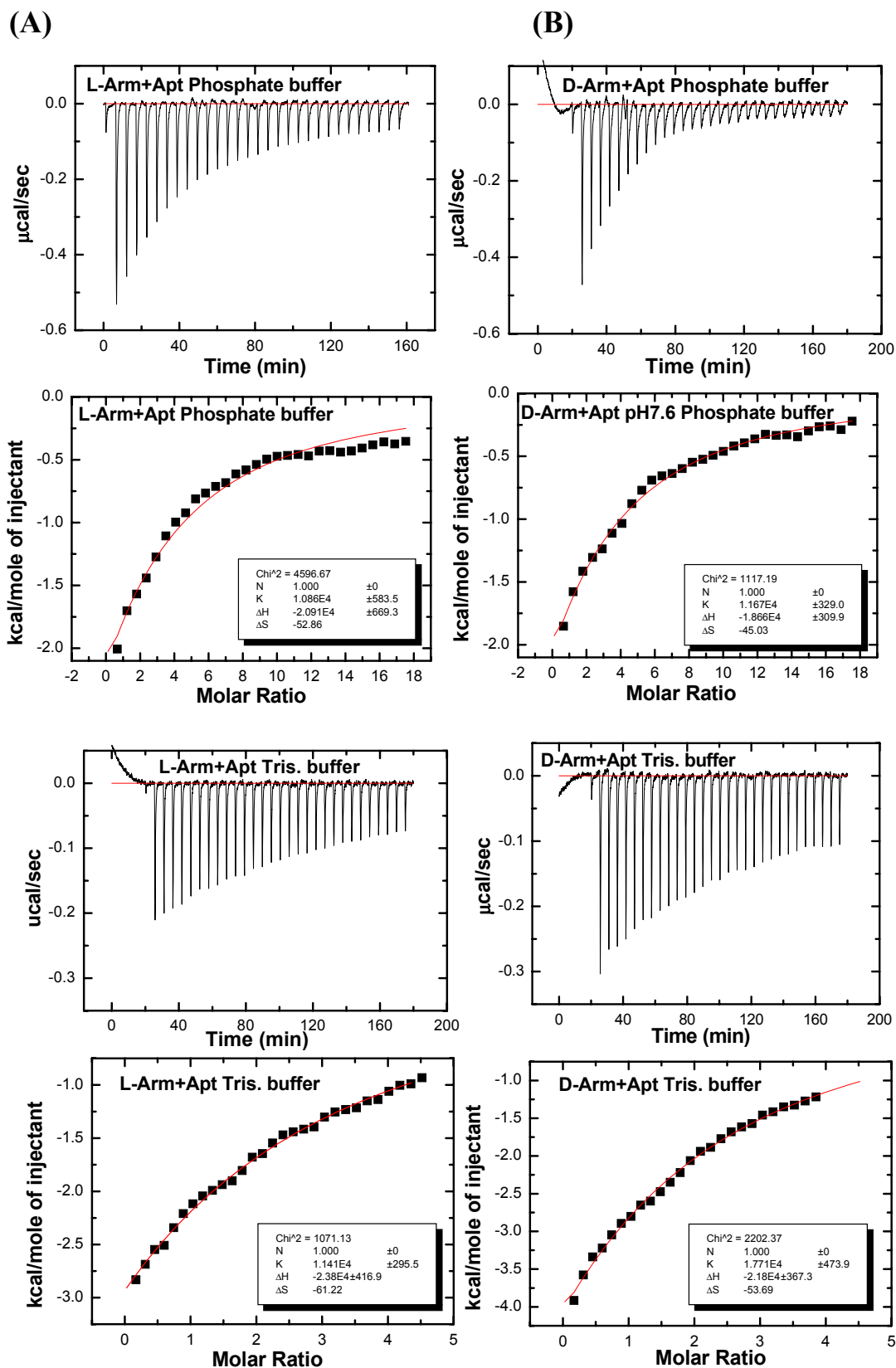
Figure S4. The ITC profiles at 10mM phosphate & Tris buffer, 100mM NaCl, pH 7.6, 20°C (A) L-Arm (B) D-Arm
