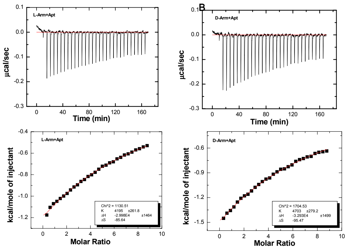
Figure S1. The ITC profiles at 10mM phosphate buffer, 25mM NaCl, pH 6.5, 20°C (A) L-Arm (B) D-Arm
