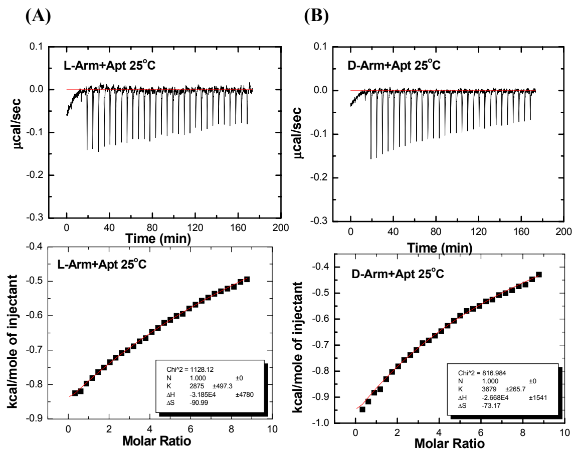
Figure S2. The ITC profiles at 10mM phosphate buffer, 25mM NaCl, pH 6.5, 25°C (A) L-Arm (B) D-Arm
