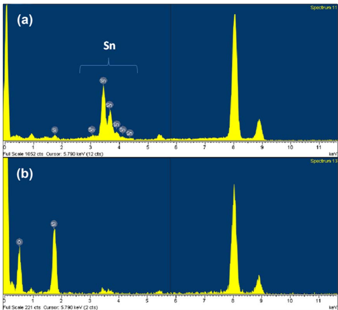
Fig. S1 EDX spectra of (a) as-prepared and (b) BOE treated nano-jellyfishes. Note that metal particles are removed by BOE treatment and Sn signal is absent accordingly. The peaks at 8 to 9 keV arise from copper grids.
