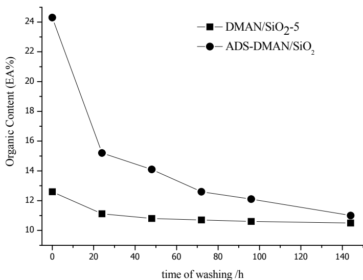
Fig. S3. Organic content vs the time of washing of the DMAN/SiO 2 -5 and ADS-DMAN/SiO 2 materials.
