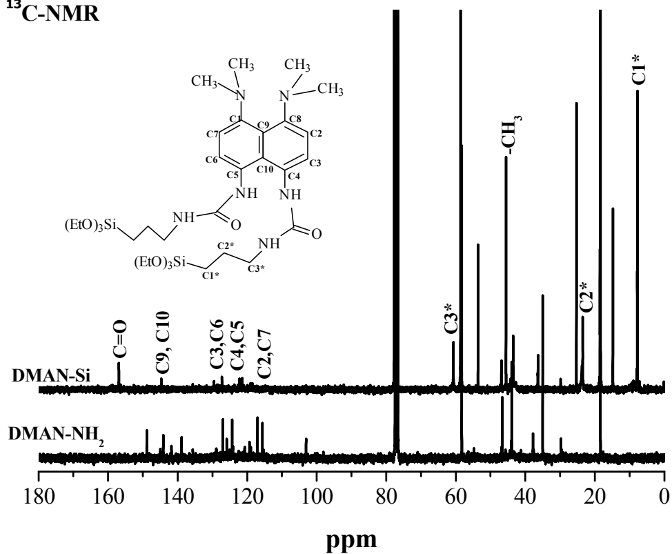
Fig. S2 – 13 C NMR spectra of DMAN-NH 2 and DMAN-Si
