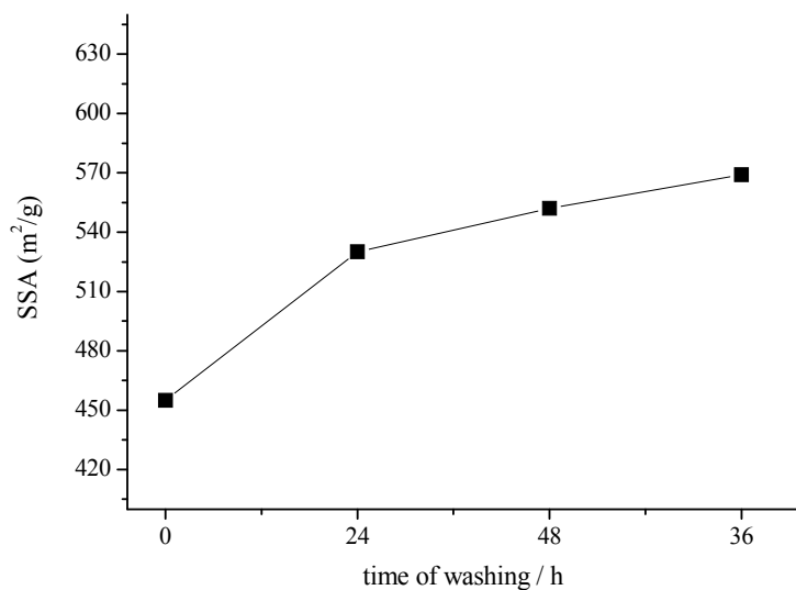
Fig.S4 – SSA vs the time of washing of the DMAN/SiO 2 -5 material.
