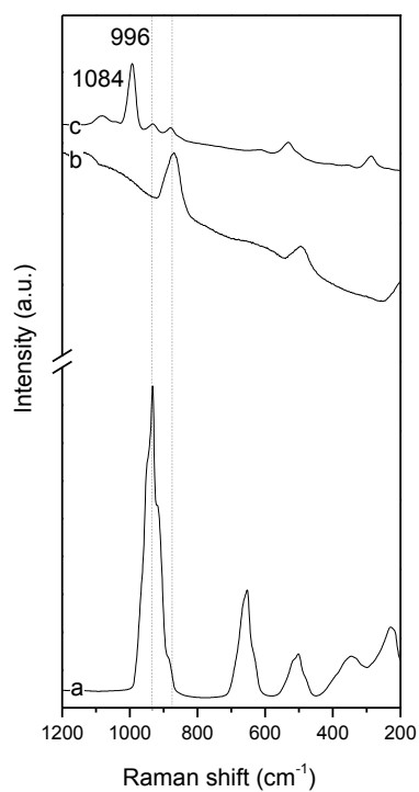
Figure S2 Raman spectra of a: \text{NH}_4\text{VO}_3 , b: (\text{COOH})_2 , c: P8V8.8P/Al
