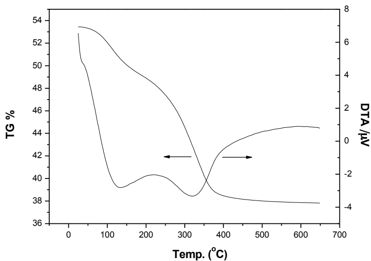
Figure S1 TG/DTG analysis of P8V8.8P/Al
