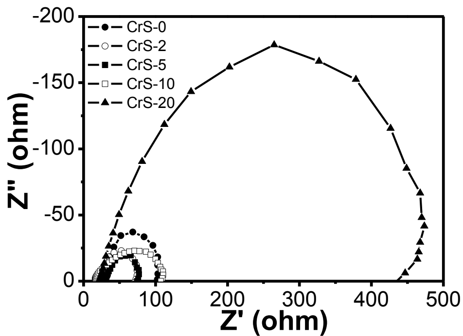
Figure S1. Electrochemical impedance spectra of DSSCs under a 100\text{mW}/\text{cm}^2 illumination
