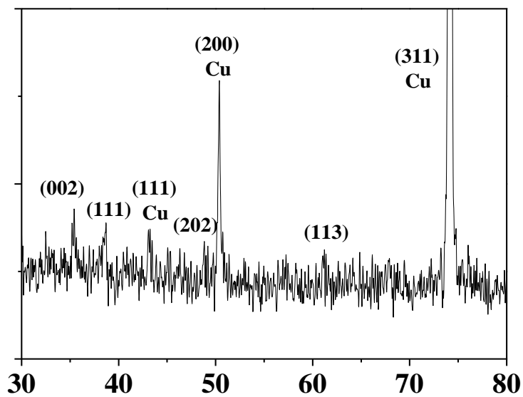
Figure S2 XRD patterns of porous CuO nanobelts
