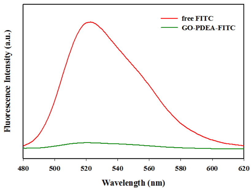
Figure S1. Fluorescence spectra of free FITC and GO-PDEA-FITC at [\text{FITC}] = 1 \mu\text{M} .
