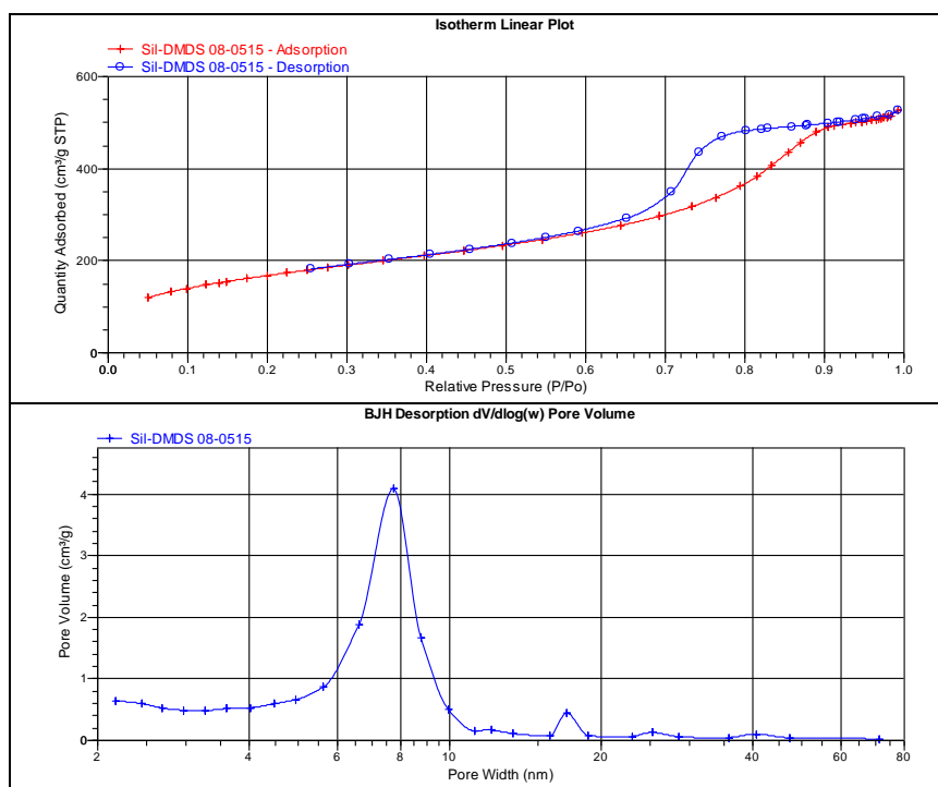
Figure SI : Adsorption/desorption isotherm and, porous distribution (ca 8 nm) of functionalized silica.
