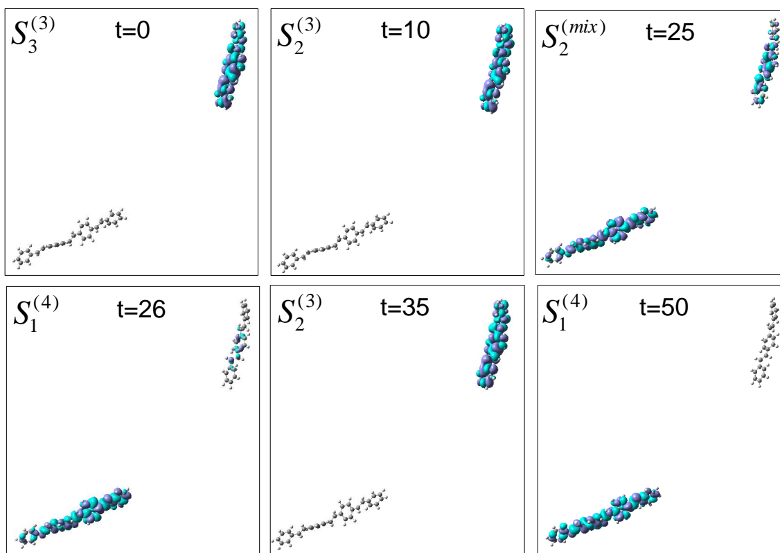
FIG. S2: Snapshots from the S_3^{(3)} \rightarrow S_1^{(4)} trajectory revealing the localization of the transition density and the conformational configuration. The time is given in femtosecond.
