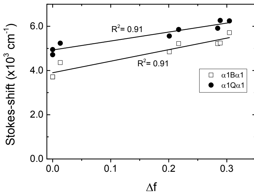
Figure S1- The lines represent a fit of the data according to the Lippert–Mataga relationship (see equation 2 in the manuscript and associated text) by using a linear regression fit.
